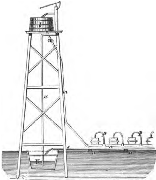
Fig. 306.—Boucherie's method of injection.
